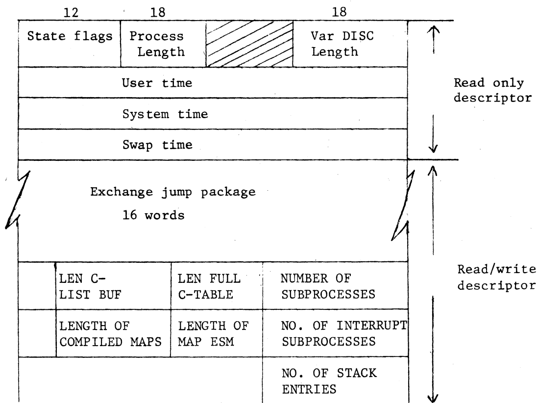
Figure 9 Display of Fixed Length Process Descriptor
